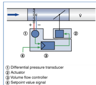
Principle of operation – Universal TROX/ Gruner
