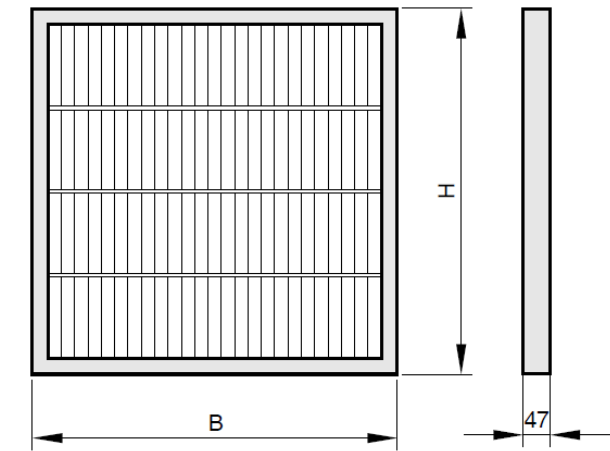
ZL, 92mm Dimensions
