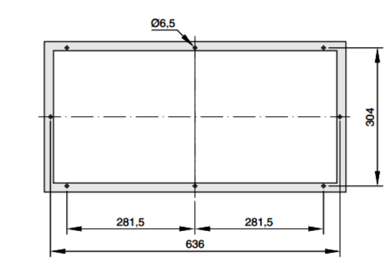
TFW flange dimensions
